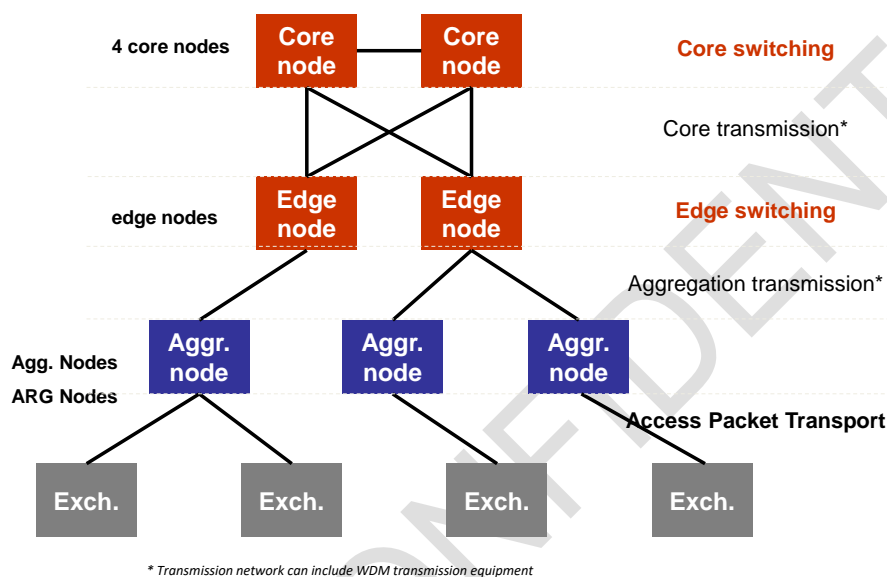
Figure 18: Overview of Eircom’s NGN
