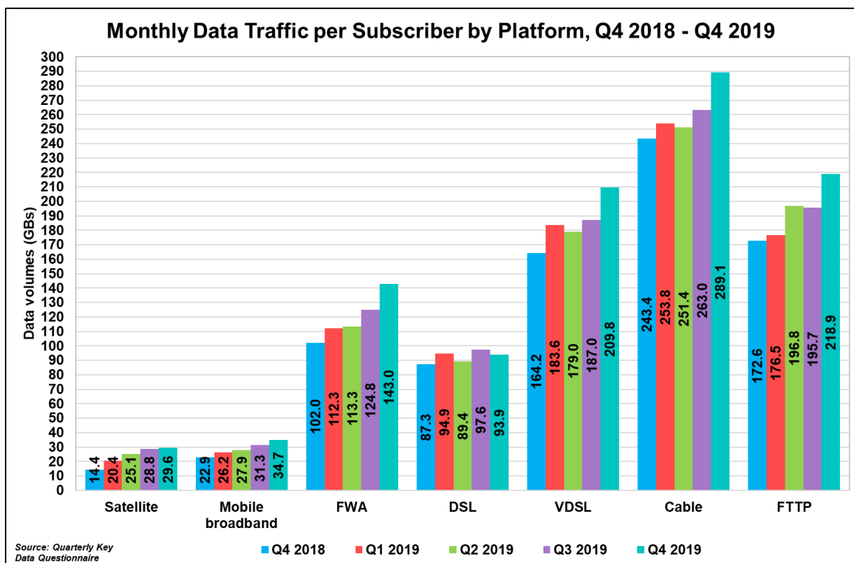
Figure 3.4.3 – Monthly Traffic per Broadband Subscription by Platform 44
