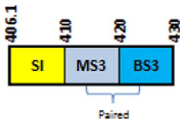
Figure 4.2: 400 MHz channel plans (Source: 25-08)
