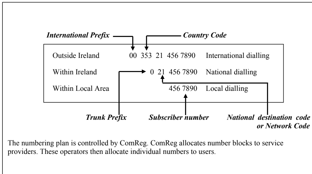
Figure 4: The different PSTN numbering terms and dialling procedures used in Ireland
