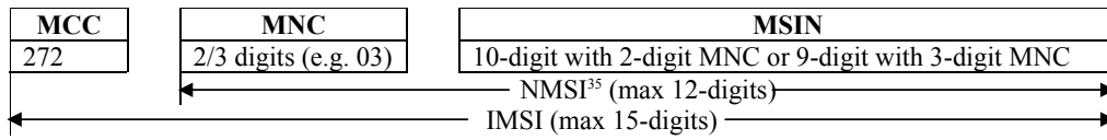
Figure 4: The structure of the IMSI
