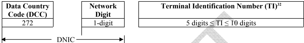
Figure 5: The structure of the DNIC and terminal identifiers
