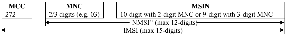
Figure 4: The structure of the IMSI
