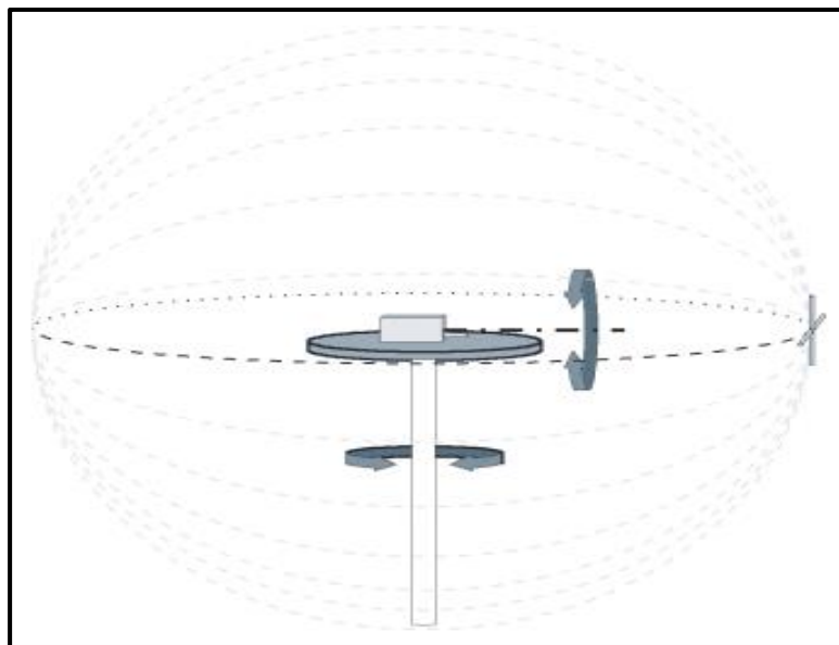
Figure 6: The great circle cut method
