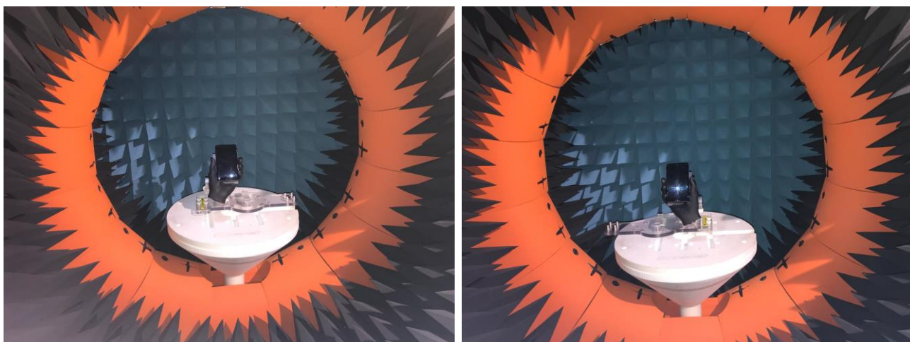
Figure 2: Handset Positioning for HL (left) and HR (right) scenarios
