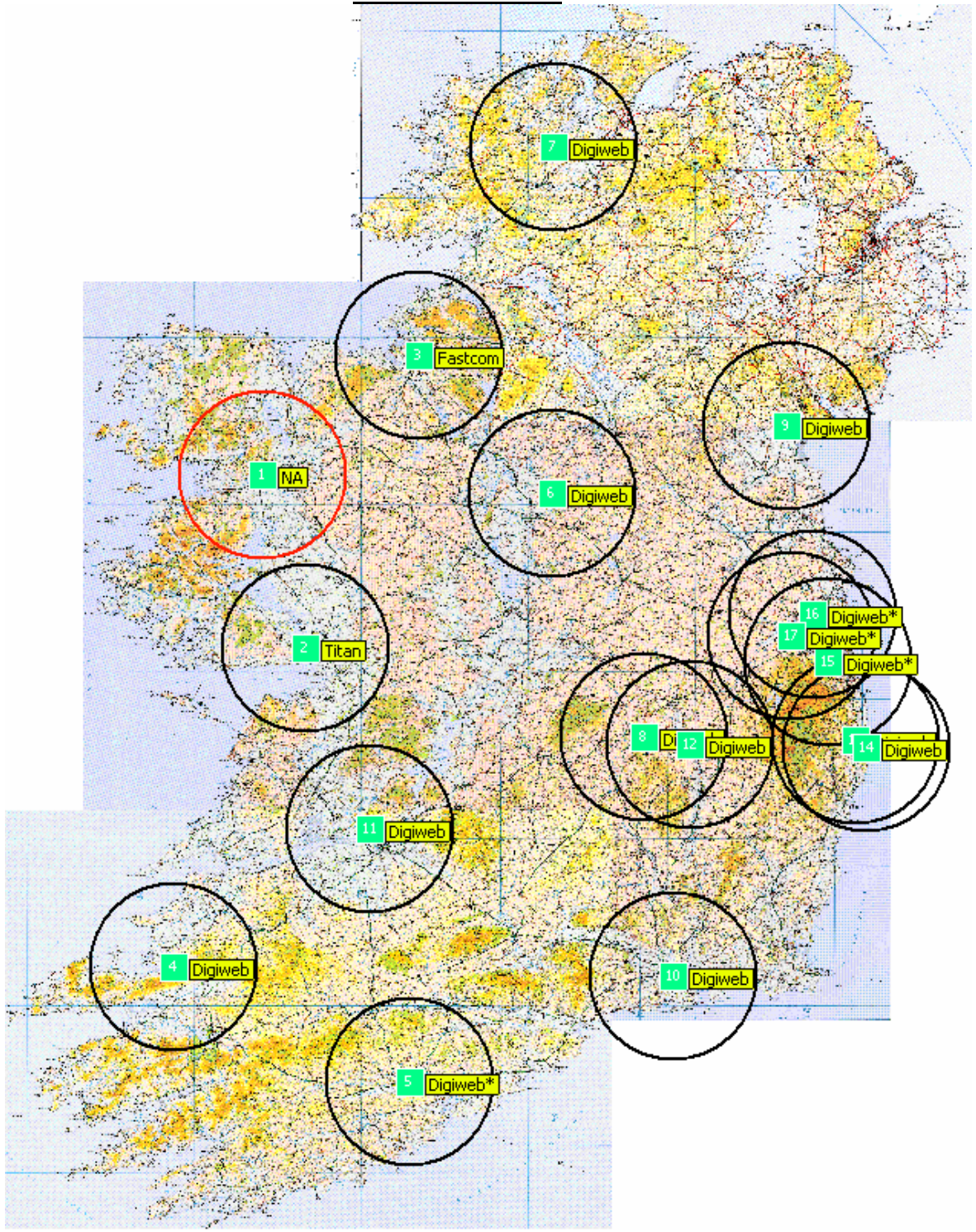
Figure 3: 10.5 GHz FWALA Channel D map
