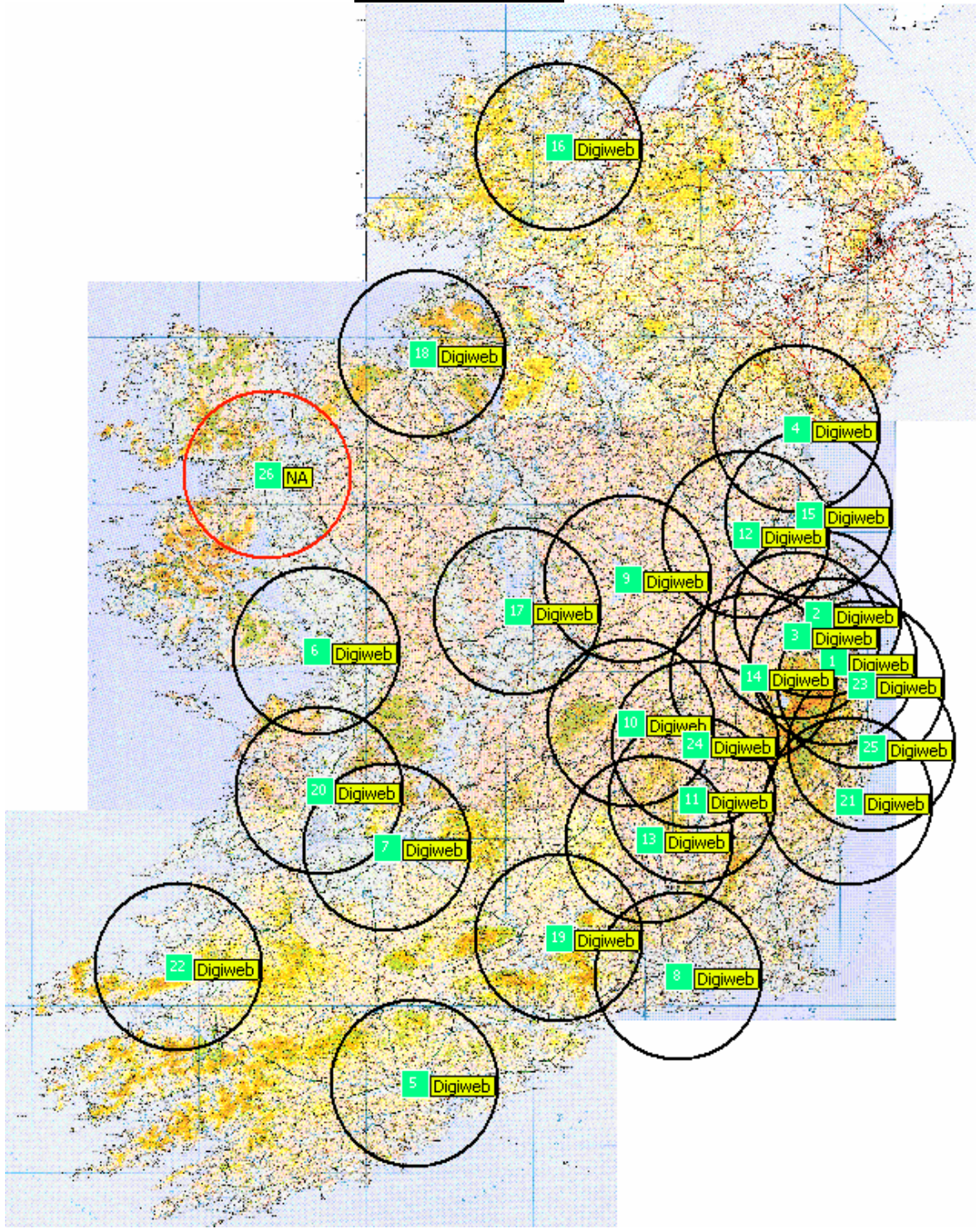
Figure 2: 10.5 GHz FWALA Channel C map
