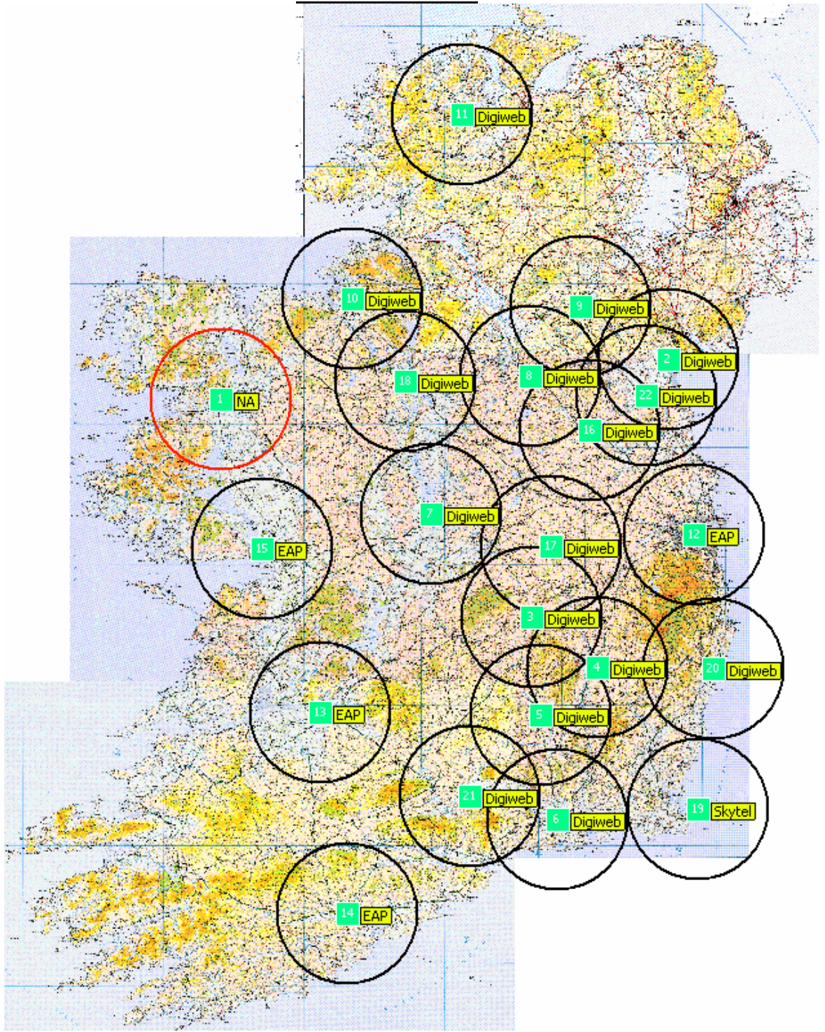
Figure 1: 3.5 GHz FWALA Channel C map
