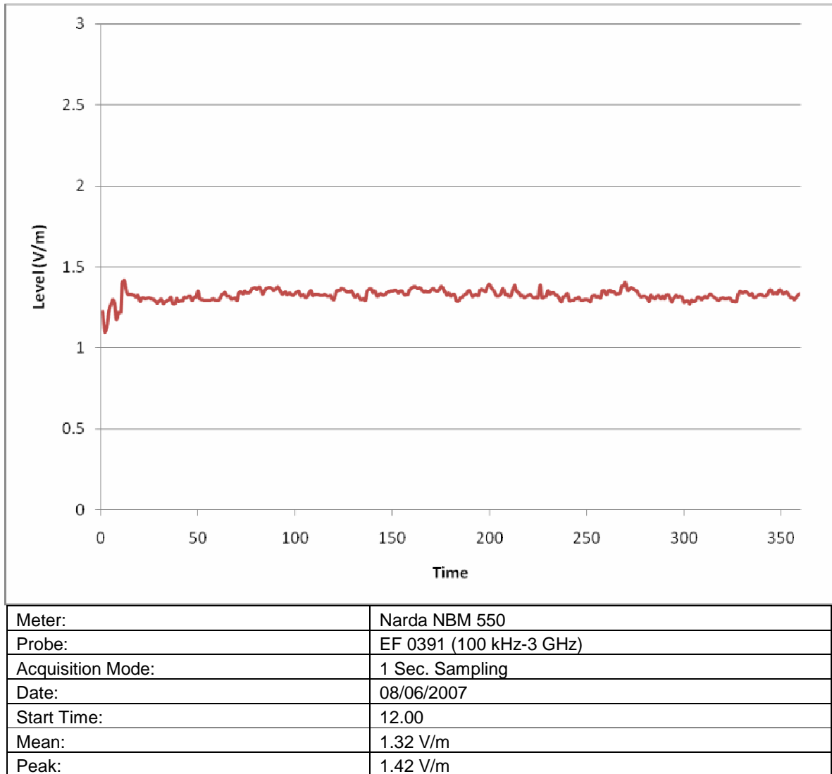
Figure 1: Field strengths recorded over a 6 minute period using the 3 GHz probe at location of full survey.
